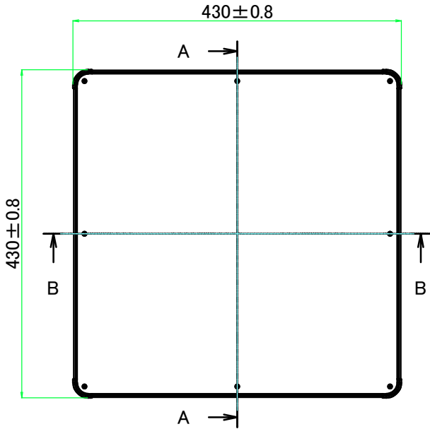
E view
