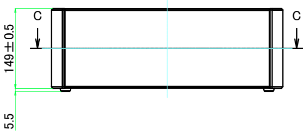
A view
